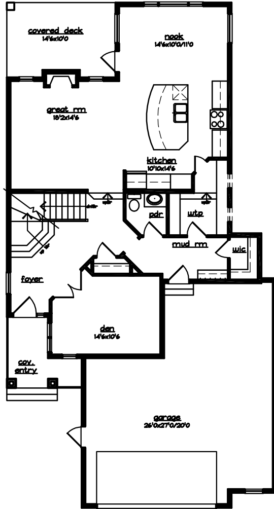
Main Floor Plan 1186 sf
