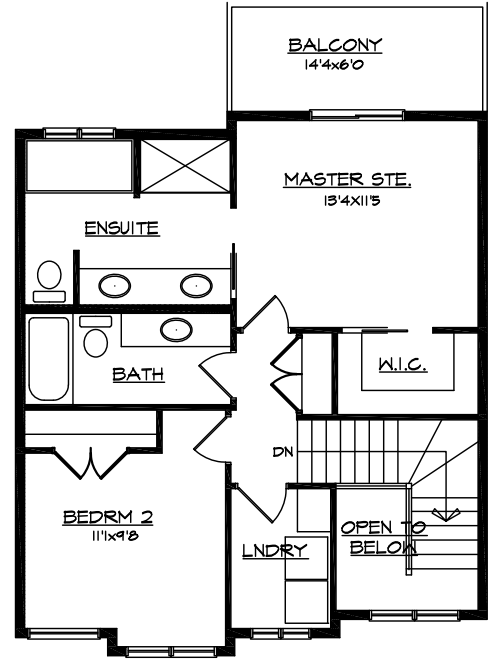
SECOND FLOOR-658 S.F..
