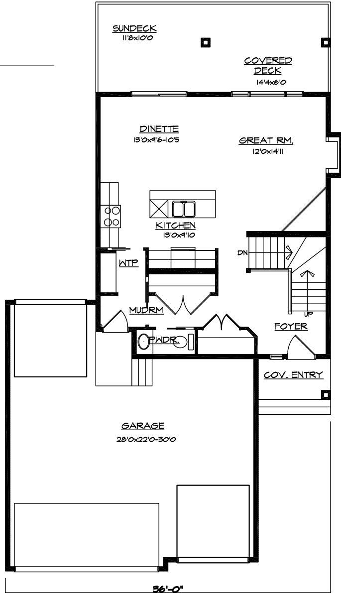
MAIN FLOOR-755 S.F.
