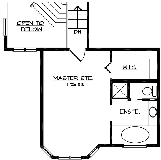
SECOND FLOOR-356 S.F.
