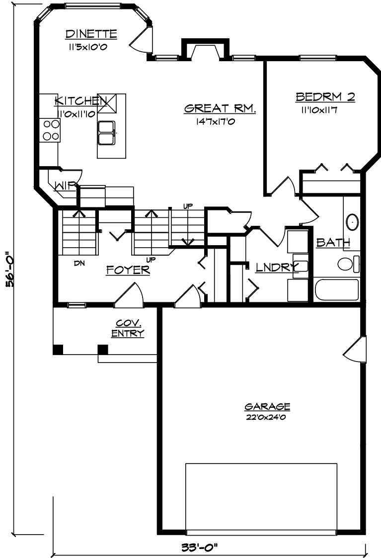
MAIN FLOOR - 986 S.F.
