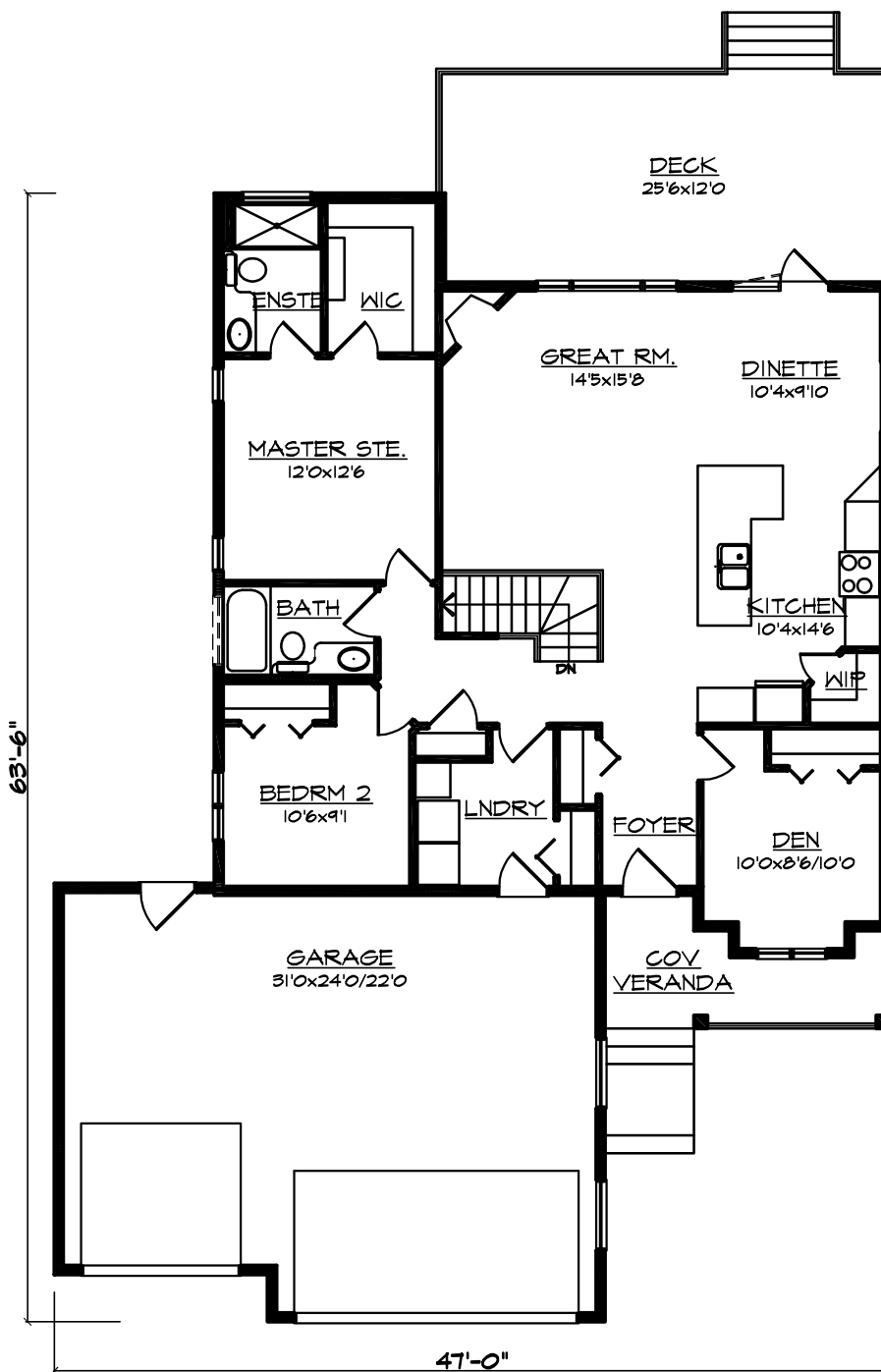
MAIN FLOOR-1409 S.F.
