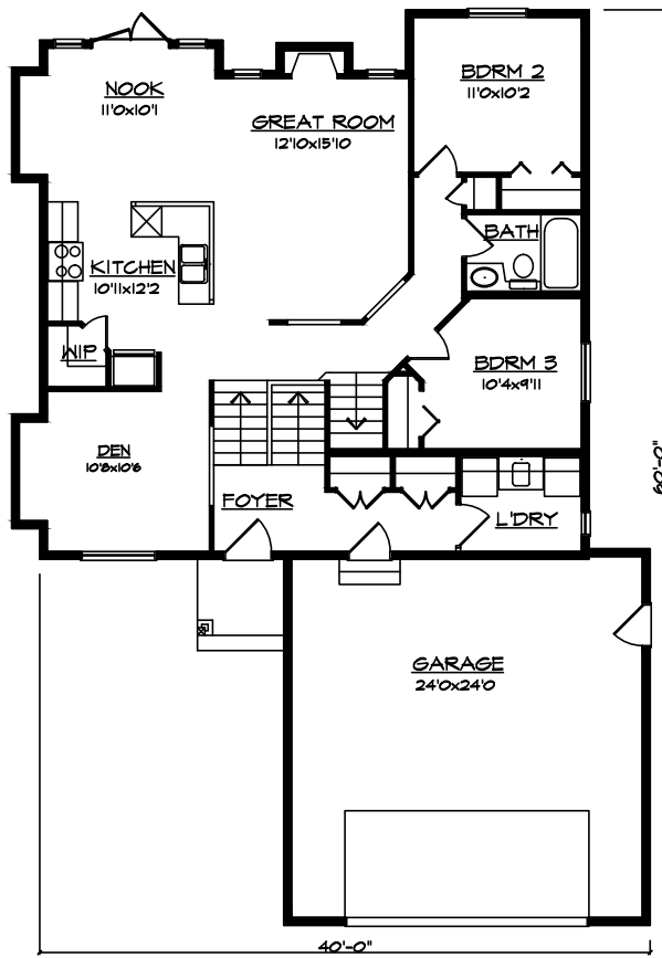
MAIN FLOOR-1224 S.F.
