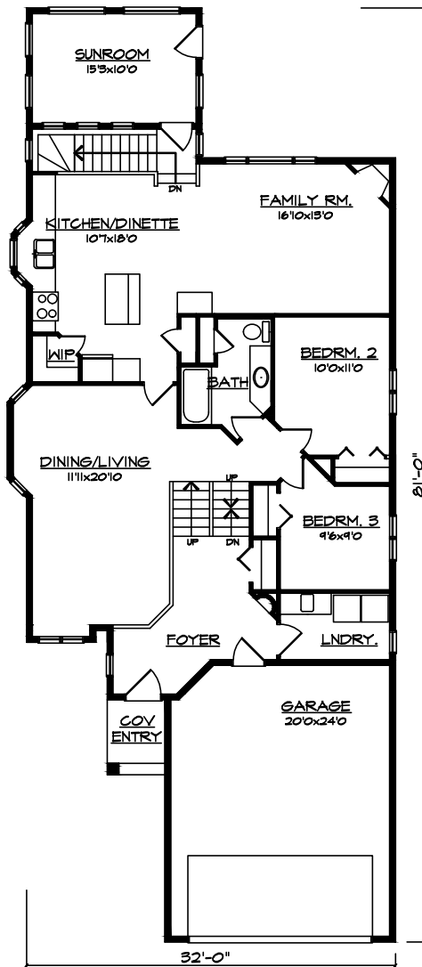
MAIN FLOOR-1476 S.F.
