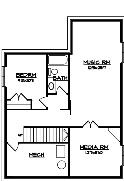
BASEMENT - 971 SF.
