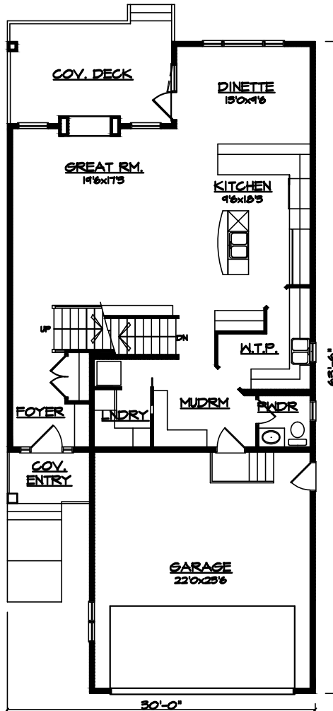
MAIN FLOOR - 1072 S.F.
