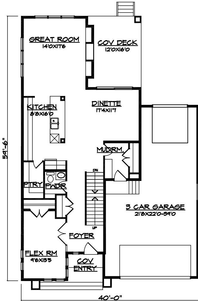
MAIN FLOOR- 1210 S.F.
