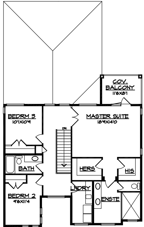
SECOND FLOOR- 1149 S.F.
