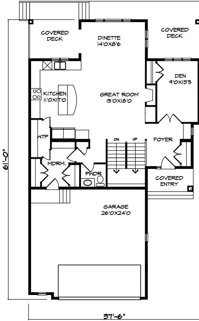
MAIN FLOOR-1131 S.F.
