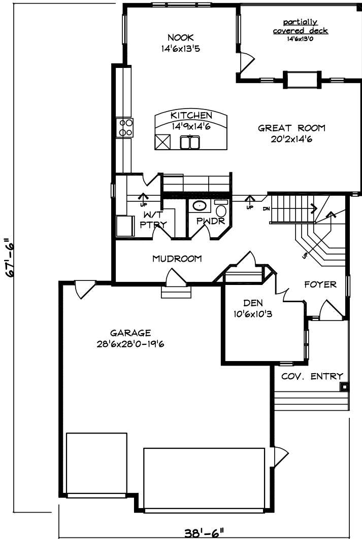
MAIN FLOOR-1201 S.F.
