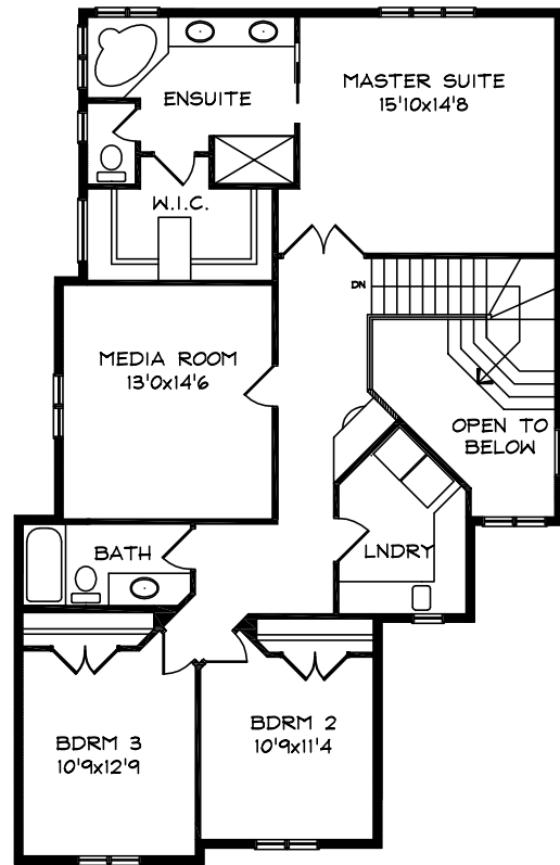
SECOND FLOOR-1324 S.F.
